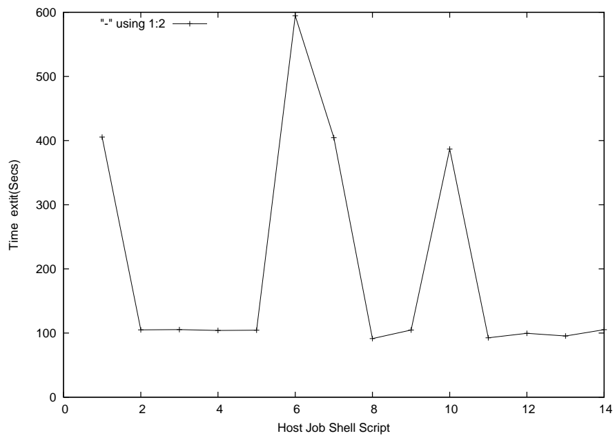
Figure 1: The Host Shell Script
