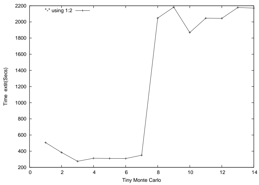
Figure 3: Tiny Monte Carlo
