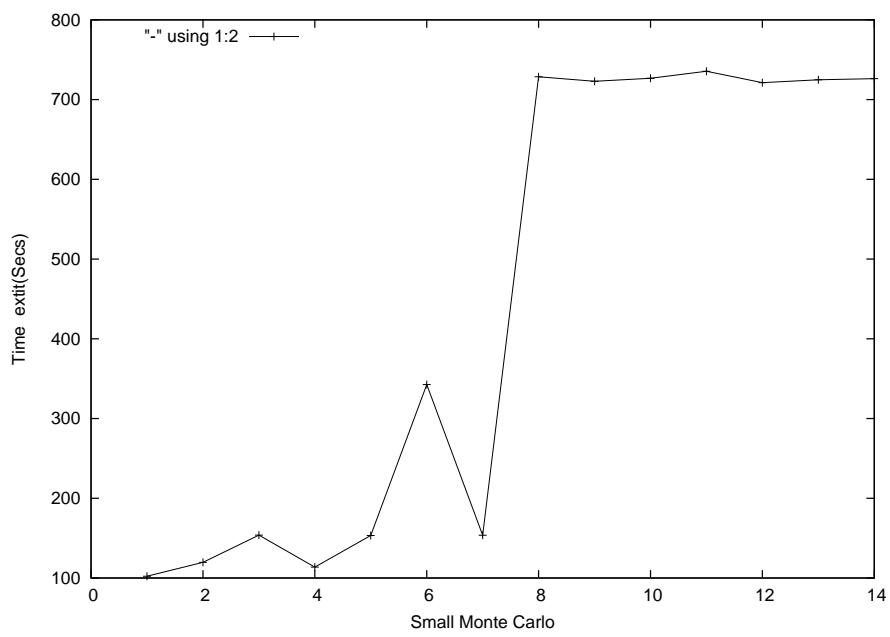
Figure 4: Small Monte Carlo
