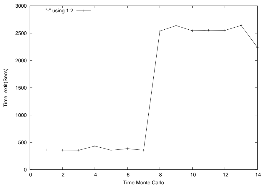
Figure 5: Time Monte Carlo
