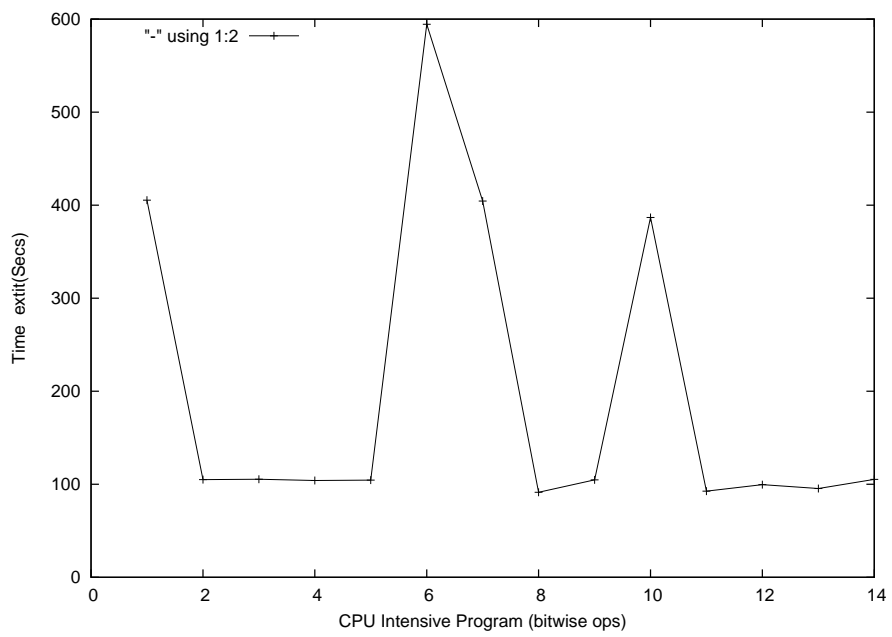
Figure 7: CPU Intensive Program (bitwise ops)
